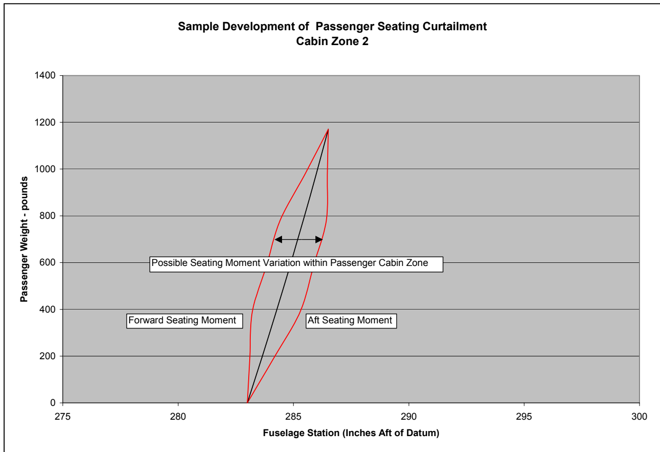
FIGURE 3-3. SAMPLE PASSENGER SEATING MOMENT (ZONE 2)
